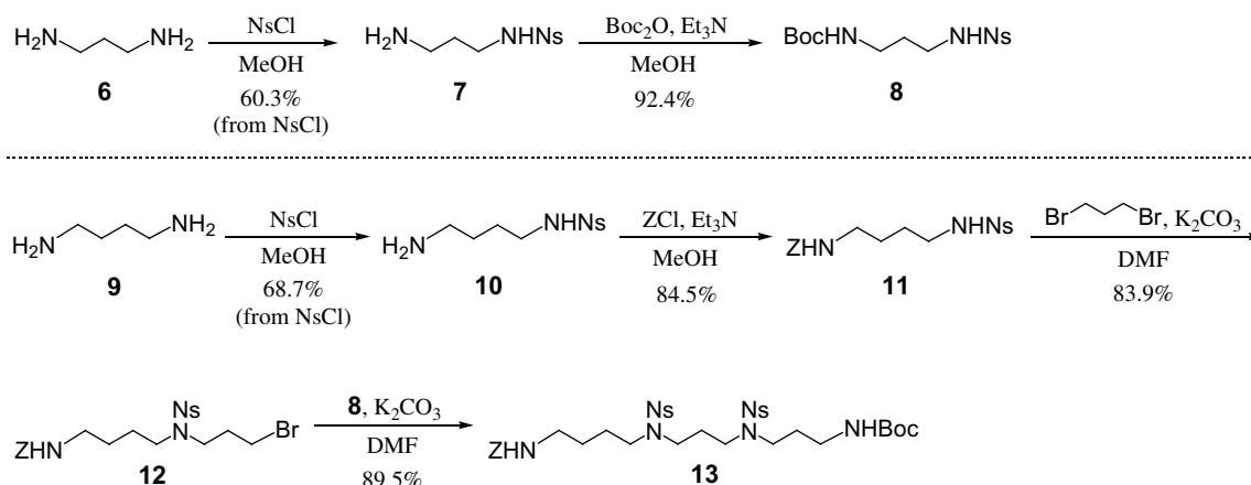
Scheme 1. Preparation of Dada derivative 13 .
